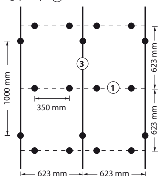
Montageprincip (A)
