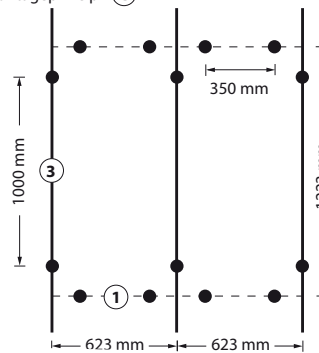
Montageprincip (C)
