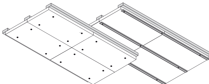
Screw (Skruvmontage)
